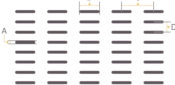
Oblong Pattern. Hole Size (A): 2mm, (B): 14mm, Pitch (C): 22mm, Pitch (D): 7mm, Open Area: 17%
