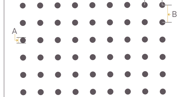
Even Pattern. Hole Size Dia (A): 1.5mm, Pitch (B): 4mm, Open Area: 11%
