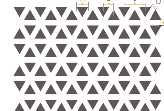
Triangular Pattern. Triangle Size (A): 10mm, Pitch (B): 9.16mm, Pitch (C): 18.32mm, (D): 4.8mm, Open Area: 30%
