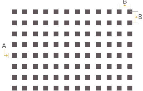
Straight Line Pattern. Hole Size (A): 4mm, Pitch (B): 9mm, Open Area: 20%
