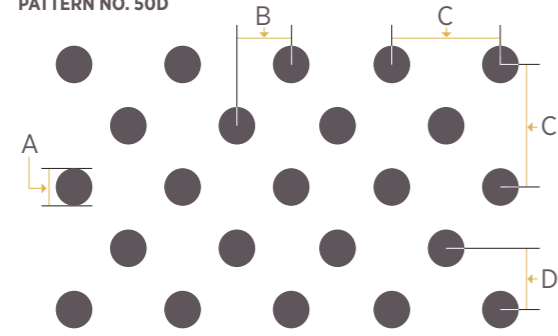
Diagonal Pattern. Hole Size Dia (A): 5mm, Pitch (B): 5mm, Pitch (C): 10mm, Pitch (D): 7.5mm, Open Area: 32%
