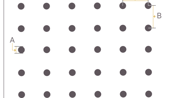
Even Pattern. Hole Size Dia (A): 2.5mm, Pitch (B): 5.5mm, Open Area: 16%
