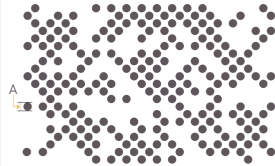
Braille Pattern. Hole Size Dia (A): 30mm, Open Area: 36%
