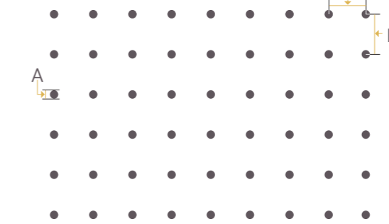
Even Pattern. Hole Size Dia (A): 0.75mm, Pitch (B): 5mm, Open Area: 1%
