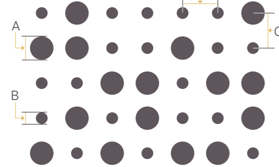
Braille Pattern. Hole Size Dia (A): 32mm, (B): 16mm, Pitch (C): 40mm, Open Area: 30%
